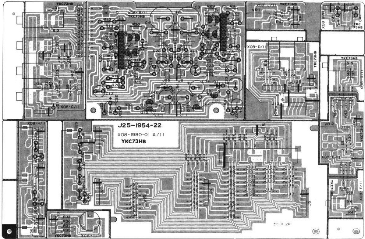
PRE AMP (X08-1980-10) Component side view
